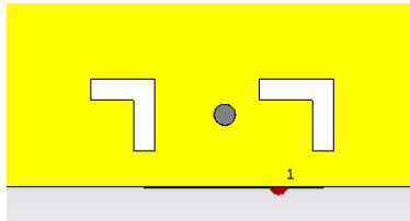
Figure 4. Two L-slots on ground plane (back view)
