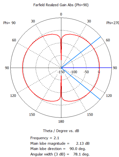
Figure 14. Simulated 2-D radiation pattern of single-dipole antenna for 2.1 GHz
