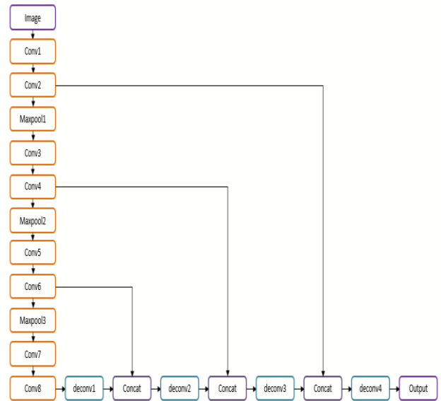
Figure 6. The detailed architecture of each Siamese branch
