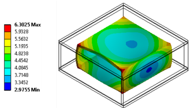
Figure 4. FEA results of the proposed reservoir of drug delivery applications
