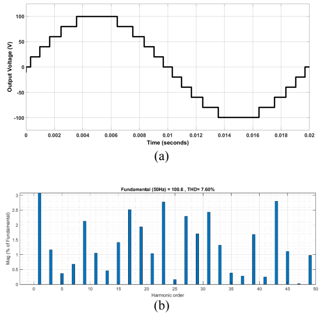
Figure 6. Simulation results for 11-level CCSMLI with R load using NLM (a) Output voltage waveform (b) Voltage THD
