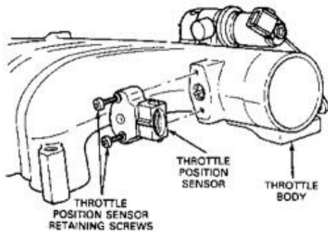
Figure 7. Throttle position sensor [4]
